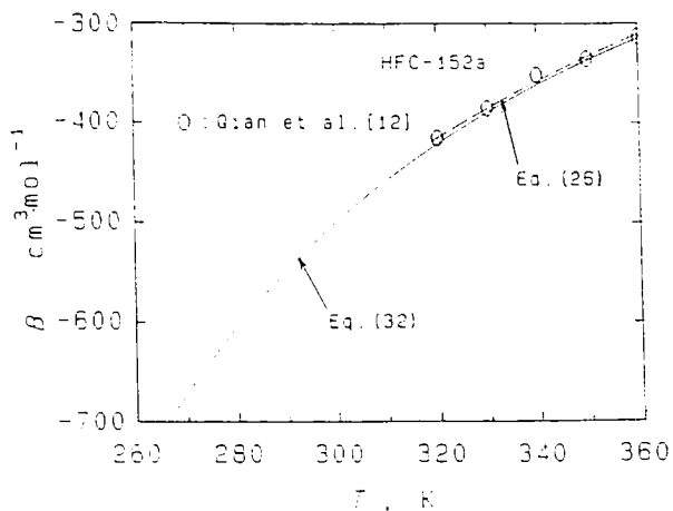
Fig. 15. Comparison with the experimental second virial coefficient values and correlations for HFC-152a.
